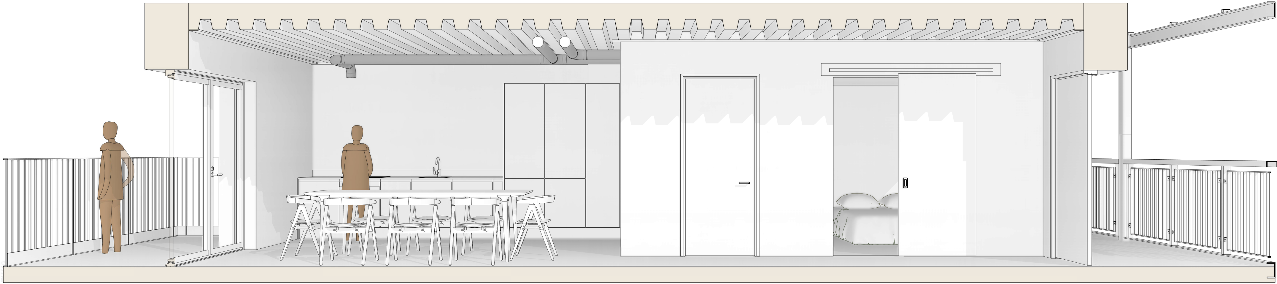
SECTION LIVING + HALL 1:25
