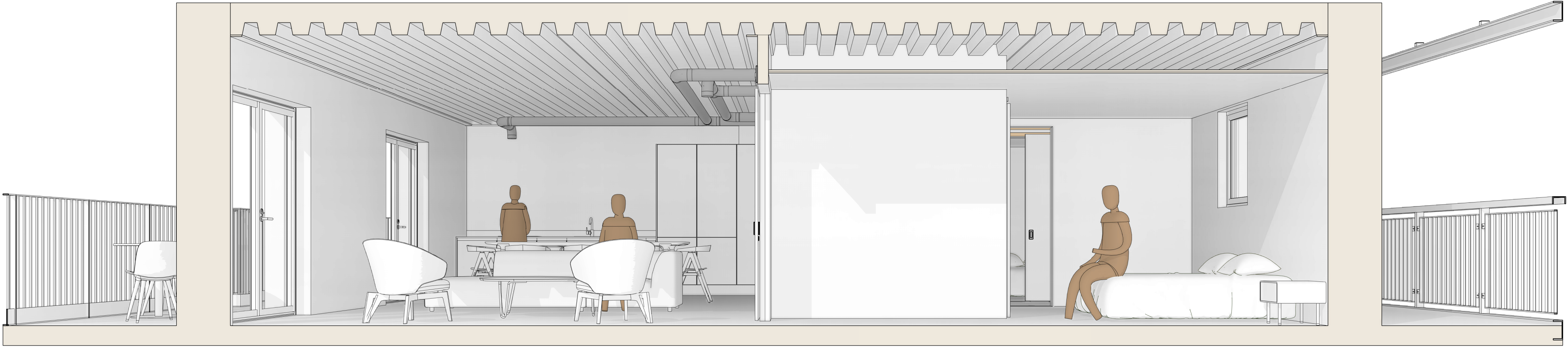
SECTION LIVING + BEDROOM 1:25
